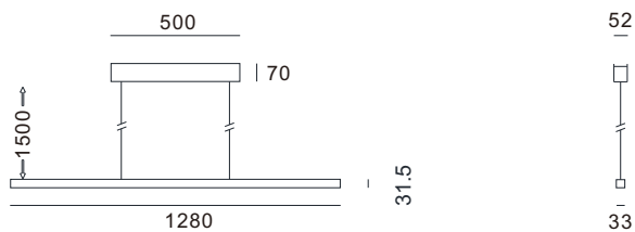
LT12 43.3W(13.5down/28.8up),5910lm(2160down/3750up),2.8kg.
