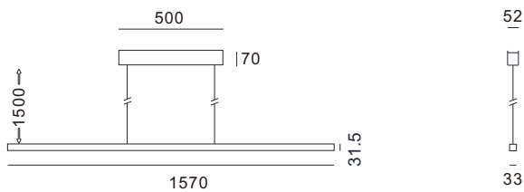
LT15 51.7W(16.5down/35.2up),7216lm(2640down/4576up),3.4kg.
