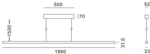
LT18 61.1W(19.5down/41.6up),8528lm(3120down/5408up),4kg.
