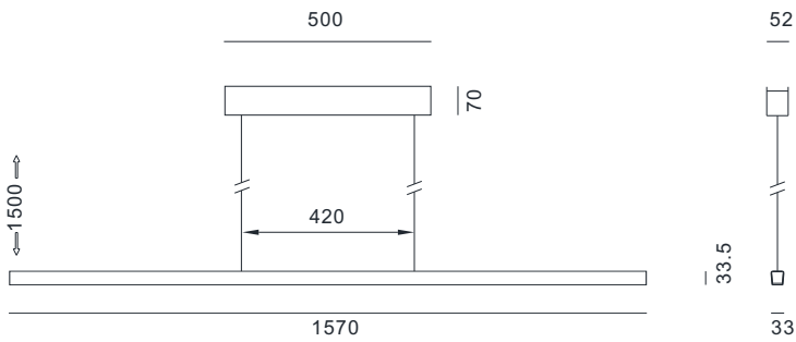
NC15 51.7W(16.5down/35.2up),7216lm(2640down/4576up),3.5kg.
