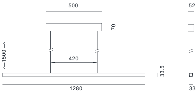
NC12 43.3W(13.5down/28.8up),5910lm(2160down/3750up),3.2kg.
