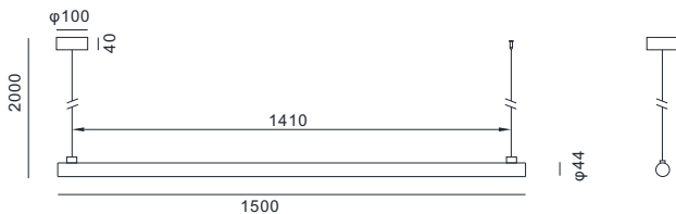
SL15 21W,Constant current 600mA 3360lm,6.6kg.
