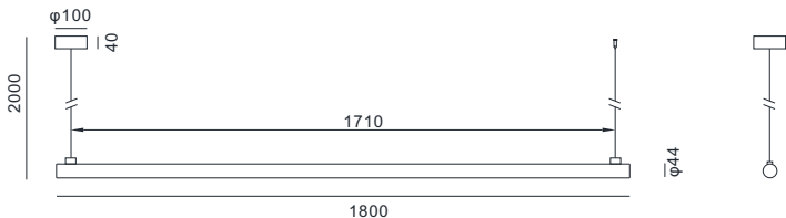
SL18 25.5W,Constant current 700mA 4080lm,8kg.
