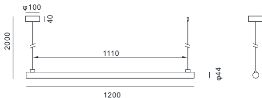
SL12 16.5W,Constant current 450mA,2640lm,5.3kg.
