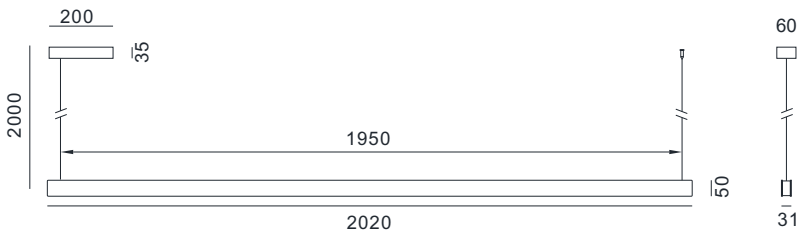
TLDN20 18W, 2880lm, 4.1kg.
