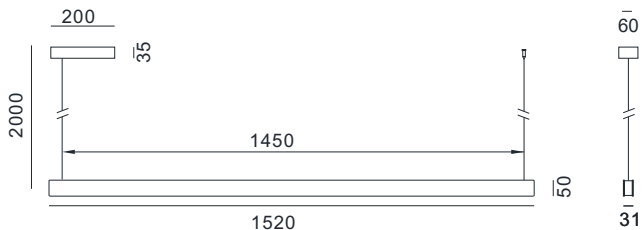
TLDN15 13.5W, 2160lm, 2.4kg.
