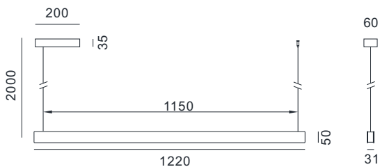
TLDN12 10.5W, 1680lm, 1.9kg.
