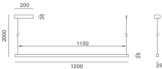
BFDN12 10.5W,1680lm,1.53kg.
