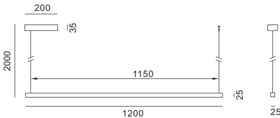
BFUP12 22.4W,2912lm,1.53kg.
