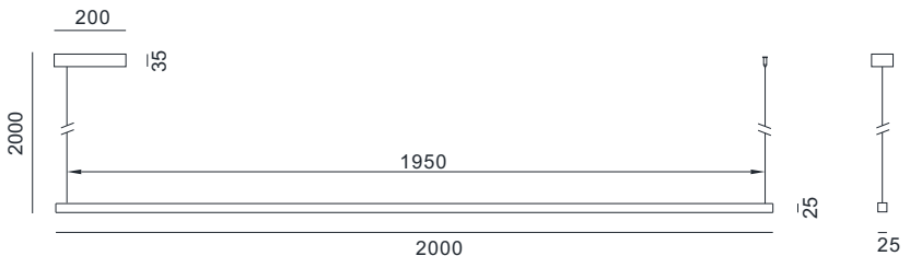
BFUP20 38.4W,4992lm,2.55kg.
