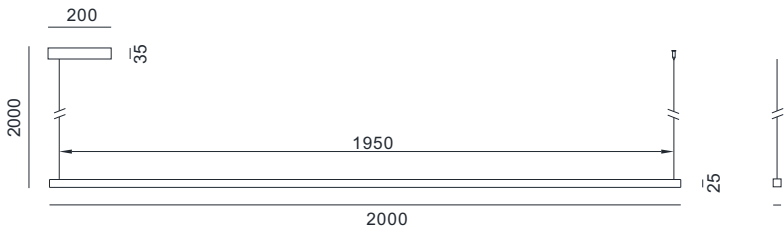
BFDN20 18W,2880lm,2.55kg.
