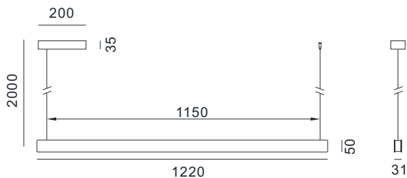
CFDU12 32.9W(10.5down/22.4up),4592lm(1680down/2912up),2.5kg.
